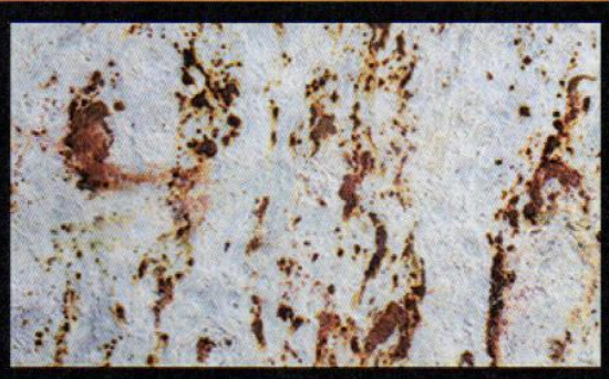
ASTM A653 G40 Compliant at 72 hours
